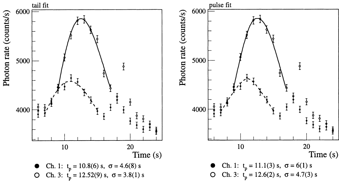
FIG. 4.—As in Fig. 2, but for GRB 980703
