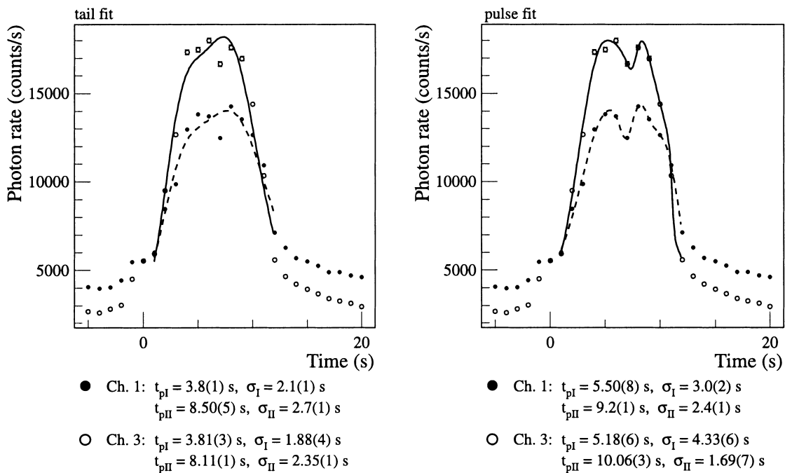
FIG. 3.—As in Fig. 2, but for GRB 980329
