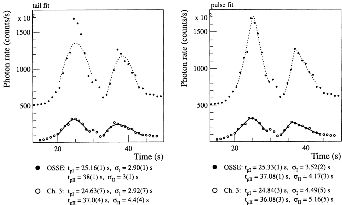
FIG. 7.—As in Fig. 6, but for GRB 990123
