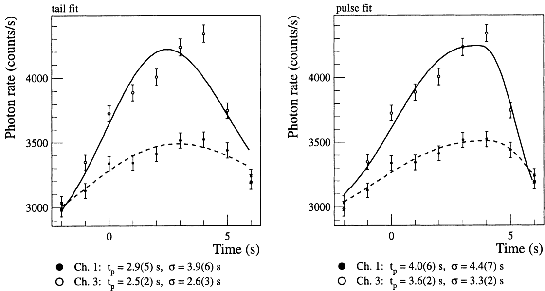
FIG. 2.—Time distribution of the number of photons observed by BATSE in Channels 1 and 3 for GRB 971214, compared with the following fitting functions: (left) “tail” function; and (right) “pulse” function. We list below each panel the positions t_p and widths \sigma_p (with statistical errors) found for each peak in each fit.
