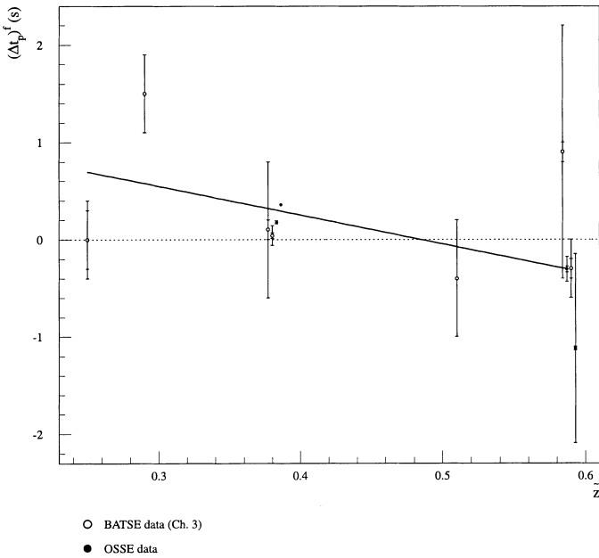
FIG. 8.—Values of the shifts (\Delta t_p)^f in the timings of the peaks fitted for each GRB studied using BATSE and OSSE data, plotted vs. \tilde{z} = 1 - (1 + z)^{-1/2} , where z is the redshift. The indicated errors are the statistical errors in the “pulse” fits provided by the fitting routine, combined with systematic error estimates obtained by comparing the results obtained using the “tail” fitting function. The values obtained by comparing OSSE with BATSE Channel 3 data have been rescaled by the factor (E_{\min}^{\text{BATSECh.3}} - E_{\max}^{\text{BATSECh.1}})/(E_{\min}^{\text{OSSE}} - E_{\max}^{\text{BATSECh.3}}) , so as to make them directly comparable with the comparisons of BATSE Channels 1 and 3. The solid line is the best linear fit.
