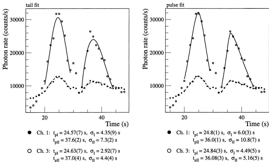
FIG. 5.—As in Fig. 2, but for GRB 990123
