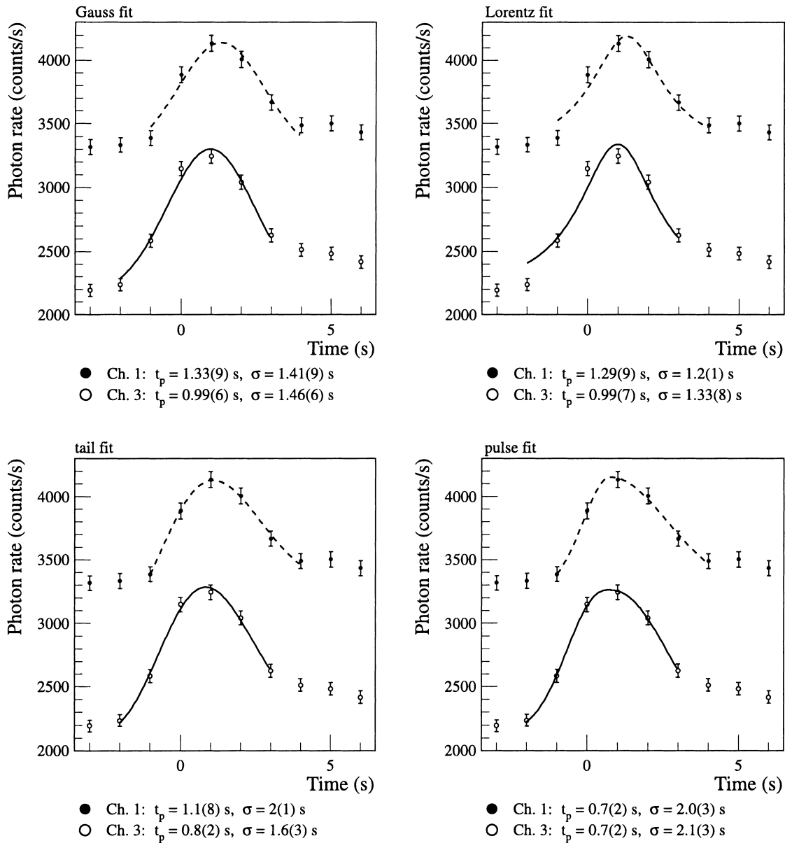
FIG. 1.—Time distribution of the number of photons observed by BATSE in Channels 1 and 3 for GRB 970508, compared with the following fitting functions: ( top left ) Gaussian; ( top right ) Lorentzian; ( bottom left ) “tail” function; and ( bottom right ) “pulse” function. We list below each panel the positions t_p and widths \sigma_p (with statistical errors) found for each peak in each fit. We recall that the BATSE data are binned in periods of 1.024 s.
