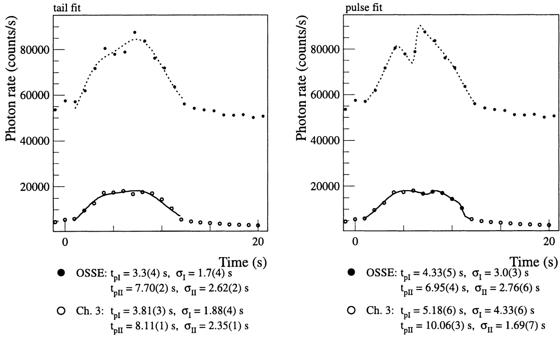
FIG. 6.—Time distribution of the number of photons observed by OSSE and by BATSE in Channel 3 for GRB 980329, compared with the following fitting functions: (left) “tail” function; and (right) “pulse” function. We list below each panel the positions t_p and widths \sigma_p (with statistical errors) found for each peak in each fit.
