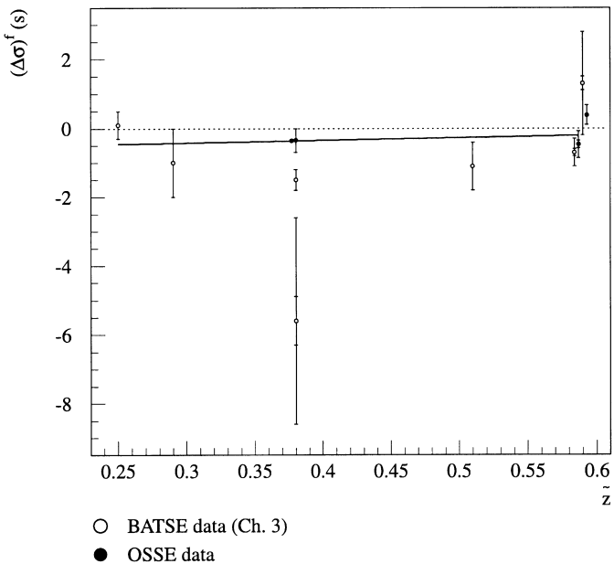
FIG. 9.—Values of the changes (\Delta\sigma)^f in the widths of the peaks fitted for each GRB studied using BATSE and OSSE data, plotted vs. \tilde{z} = 1 - (1 + z)^{-1/2} , where z is the redshift. The indicated errors are the statistical errors in the “pulse” fits provided by the fitting routine, combined with systematic error estimates obtained by comparing the results obtained using the “tail” fitting function. The values obtained by comparing OSSE with BATSE Channel 3 data have been rescaled by the factor (E_{\min}^{\text{BATSECh.3}} - E_{\max}^{\text{BATSECh.1}})/(E_{\min}^{\text{OSSE}} - E_{\max}^{\text{BATSECh.3}}) , so as to make them directly comparable with the comparisons of BATSE Channels 1 and 3. The solid line is the best linear fit.
